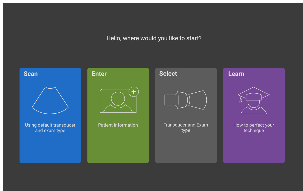
Figur 3. Startskärm
