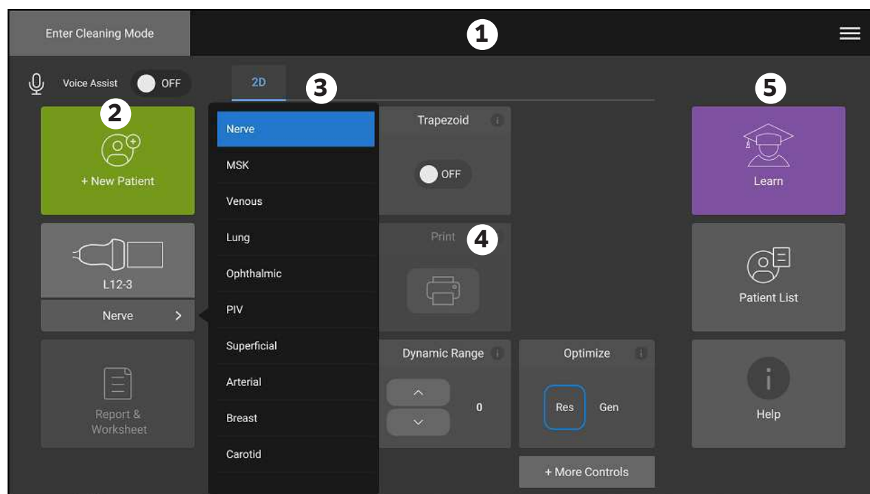
Figur 6. Pekskärmens layout
